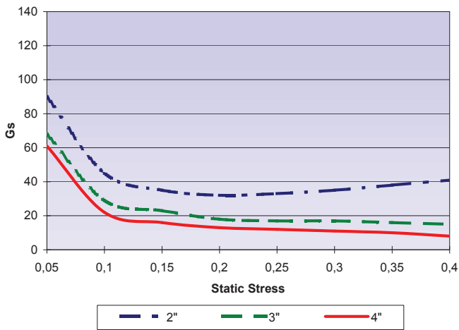
12 Inch Drop
