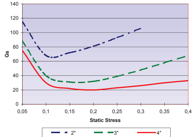
36 Inch Drop
